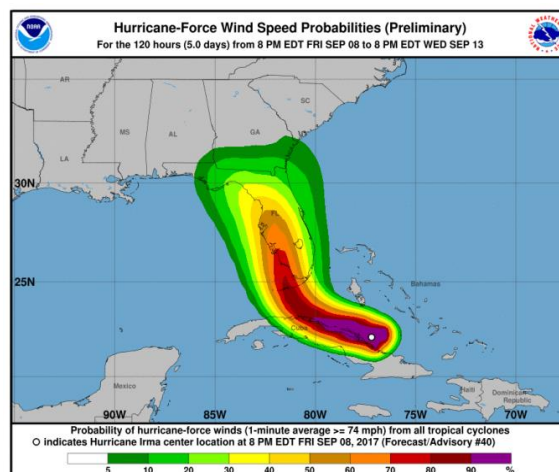
Figure 2. Range of probability of hurricane force surface winds during Hurricane Irma indicating the range of uncertainty
